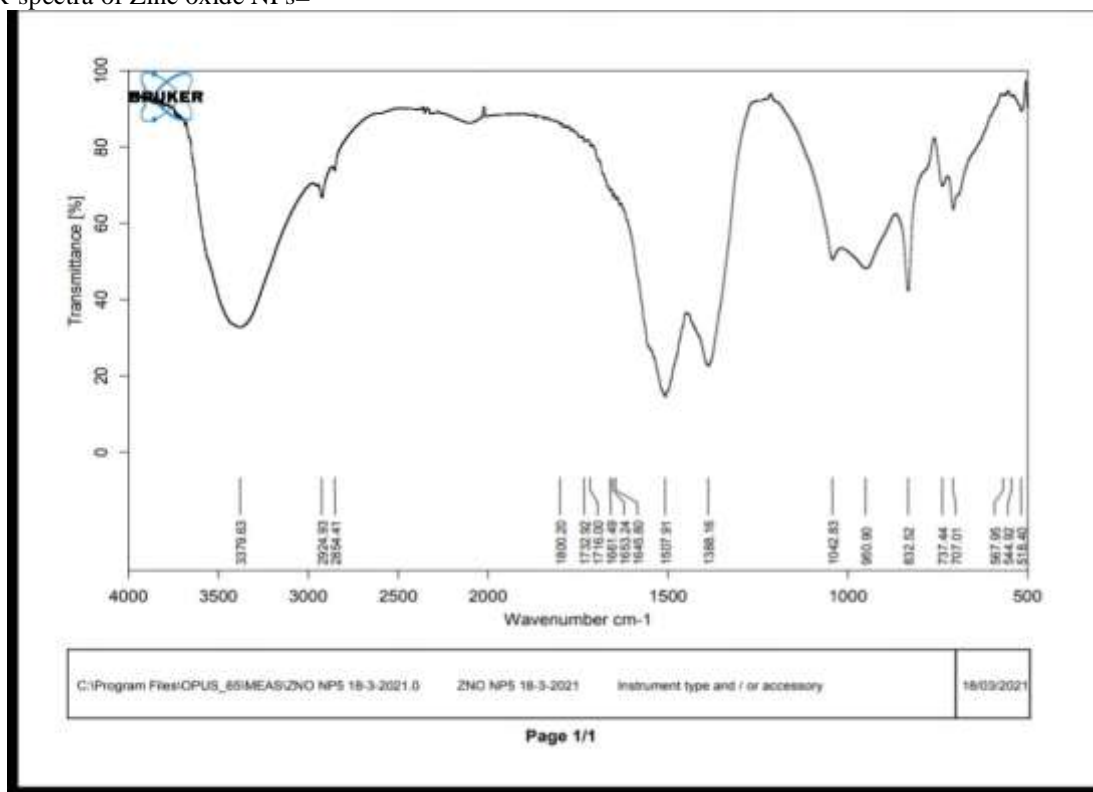
Figure-3 of FTIR-spectra analysis
