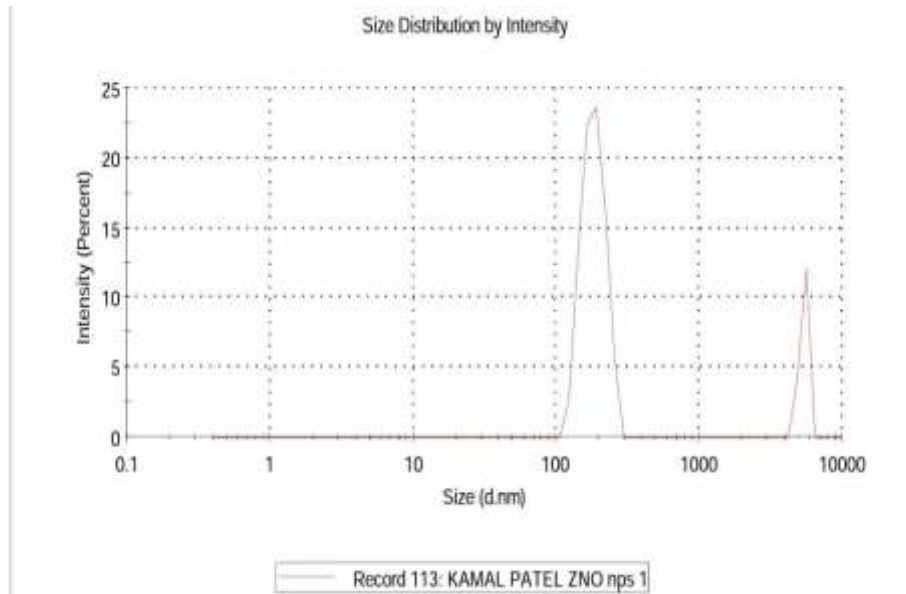
Figure-2 Particle size of the ZnO NP
