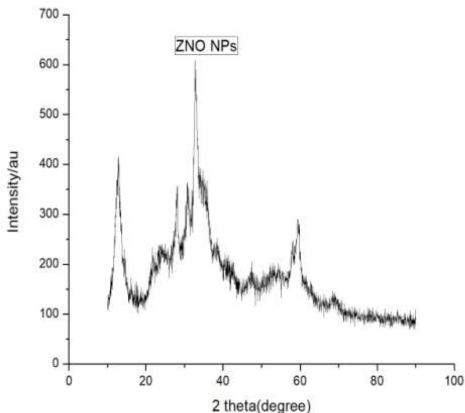
Figure-4 XRD spectra of Zinc oxide NPs
