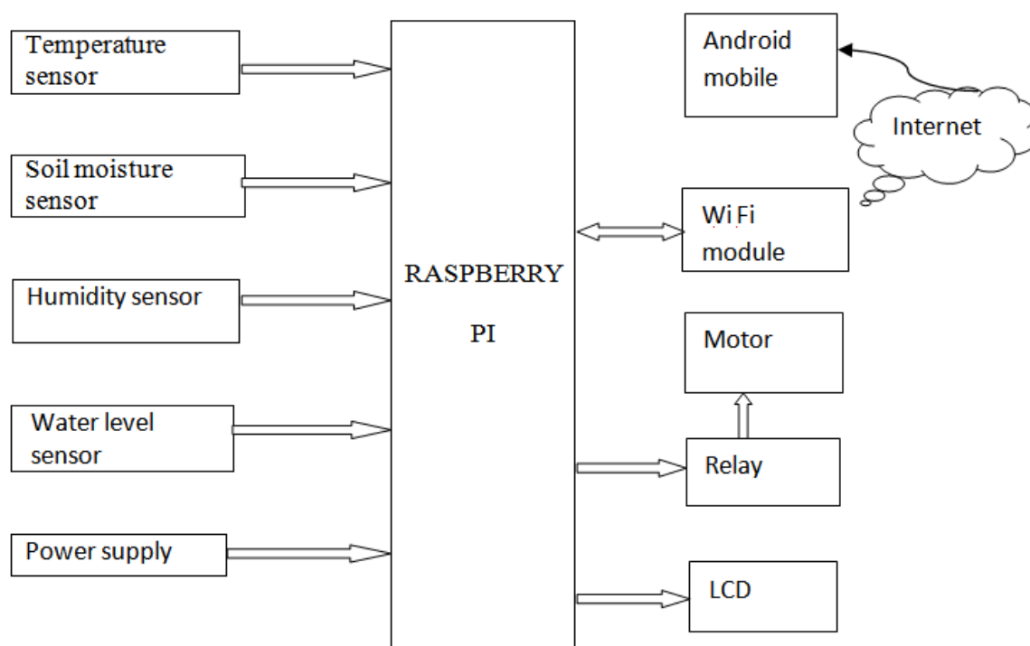
Fig: Block diagram of smart agricultural system
