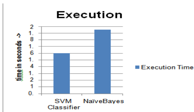
Fig. 3. Execution time
