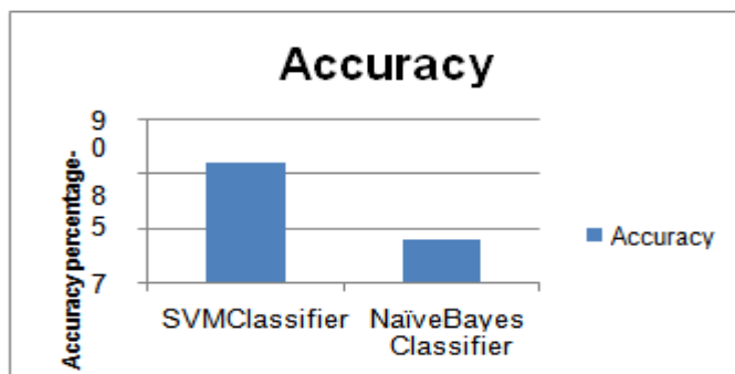
Fig. 2. Accuracy Comparisons
