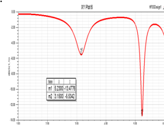
Figure 6 Return loss of patch antenna
