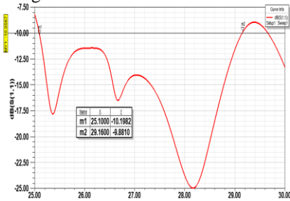
Figure 7 Return loss of proposed antenna
