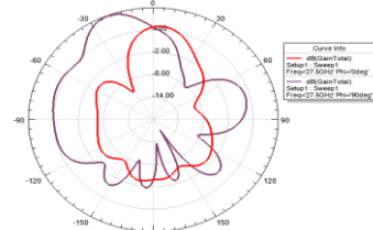
Radiation Pattern at 27.5 GHz
