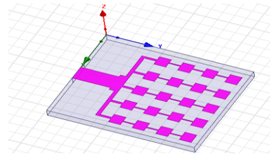
Figure 3 proposed micro strip antenna
