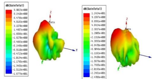
Figure 10 Gain - patch antenna
