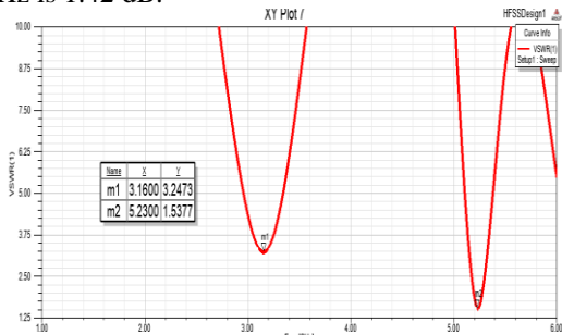
Figure 8 VSWR - patch antenna
