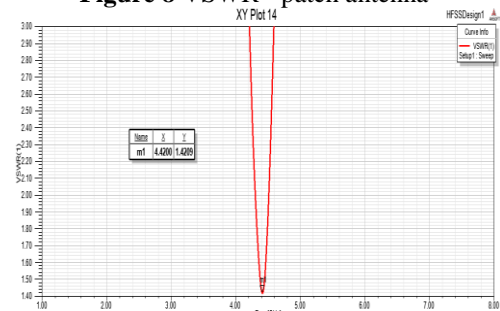
Figure 9 VSWR - array antenna
