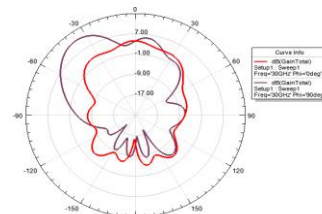
Radiation Pattern at 28.5 GHz
