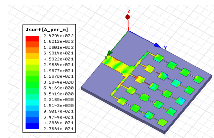
Figure 4 Current distribution in antenna
