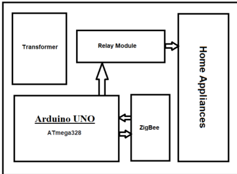
Fig 1: Receiver Circuit
