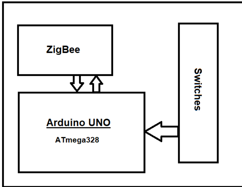
Fig 2: Transmitter Circuit
