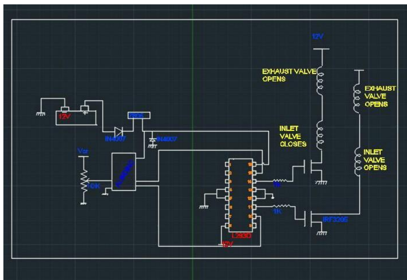
LINE DIAGRAM FOR VALVE ACTUATION OF CAMLESS ENGINE
