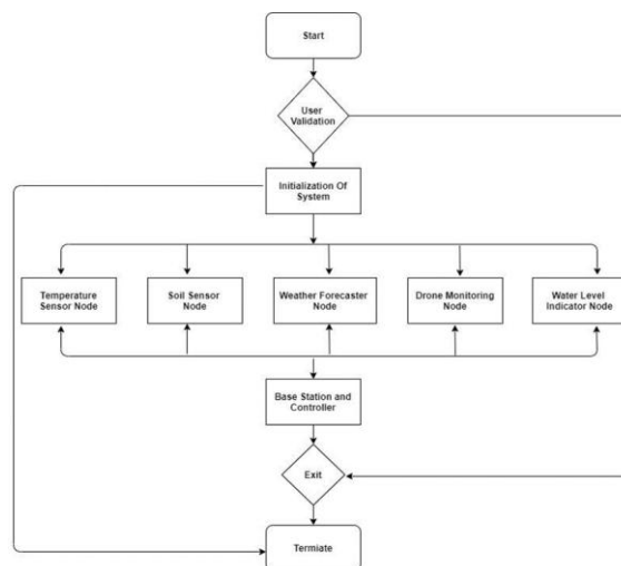
Figure 1.2: Flow Diagram
