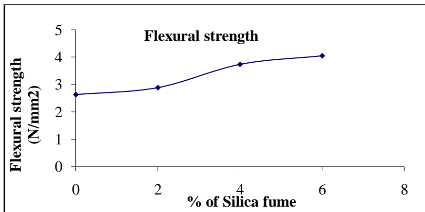
Fig 4: Effect of Silica Fume in Flexural Strength of SCC
