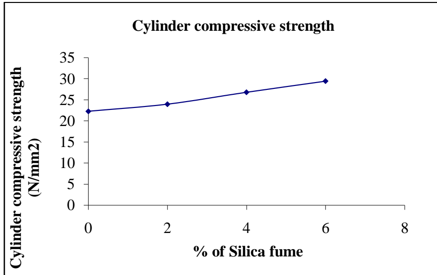
Fig2: Effect of Silica Fume in Cylinder compressive Strength
