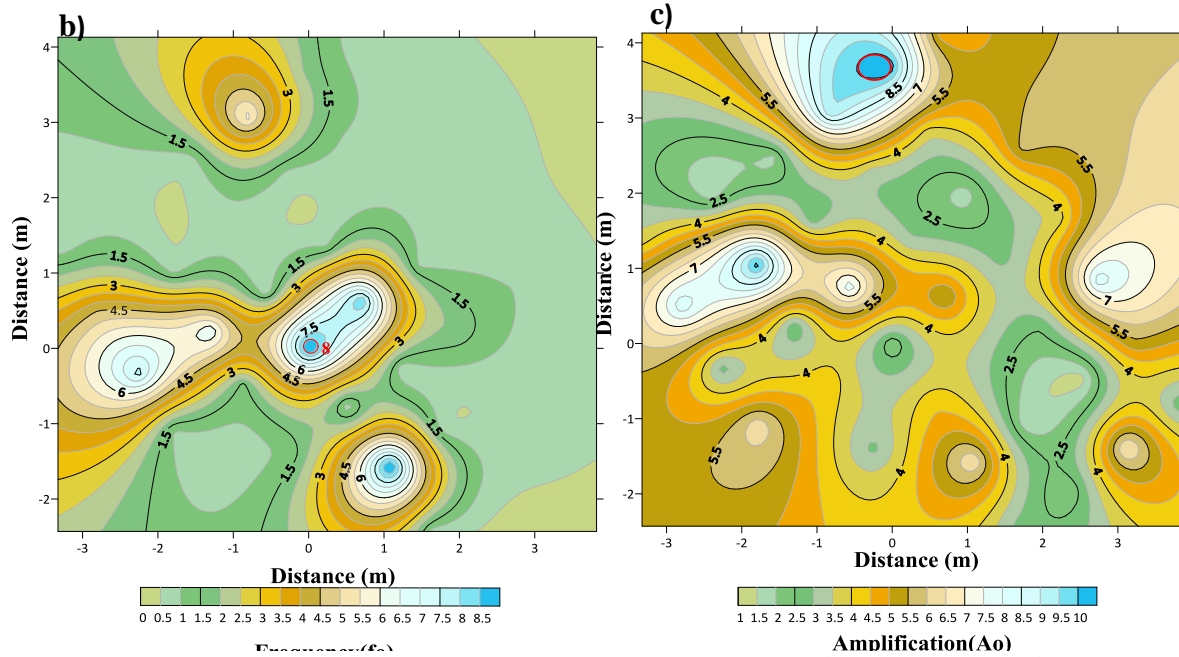
Figure 3: a) H/V overall average curve and H/V parameter; b) Distribution frequency contour (fo); c) Contour with distribution Amplification (Ao).
