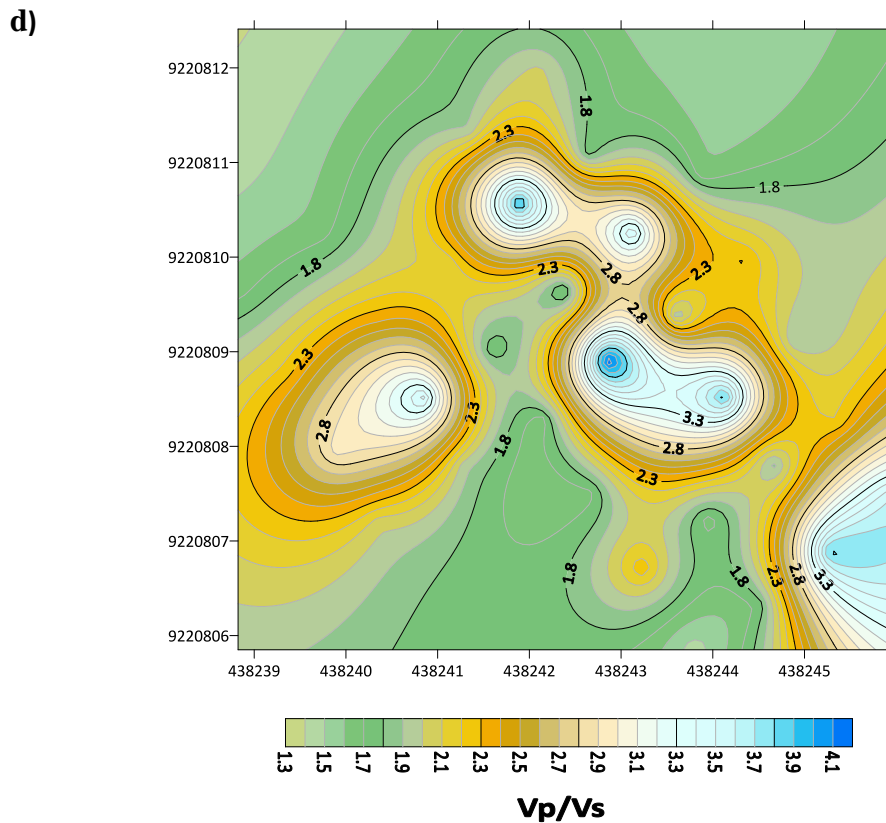
Figure4:a) Curve of Compression wave velocity; b) Curve of Shear wave velocity; c) Curve of Density; d) Curve showing the compression wave velocity by shear wave velocity
