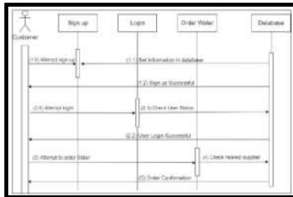
Figure 4.: Sequence Diagram
